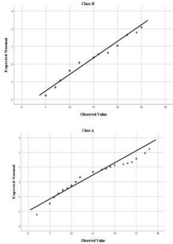
Figure 1. The quantile-quantile plot
