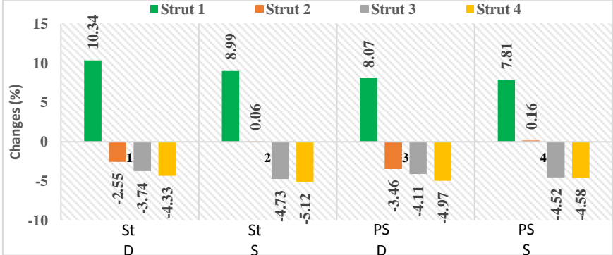
Figure 16. Strut forces changes in percent - Sand (model No.1)
