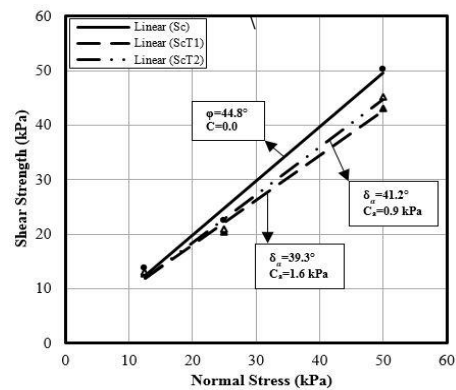
Figure 10. Failure envelopes for S_{cT1} and S_{cT2}
