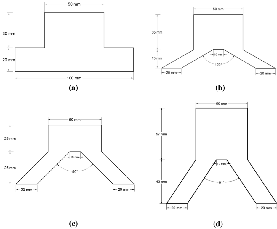
Figure 2. Geometrical configuration of footings
