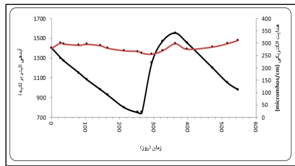
Fig. 2. Time variation of electrical conductivity and discharge in the Varskhavaran karstic spring
