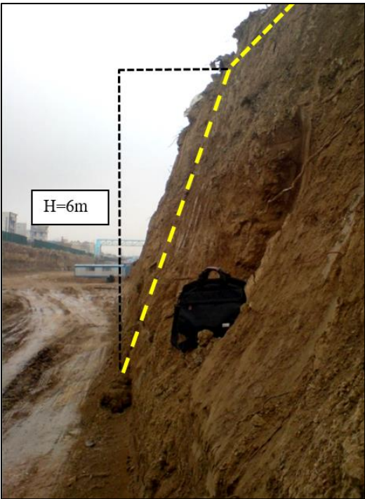
Fig. 8. The stable excavation wall with the approximate depth of 6 m and 80° in zone D 1
