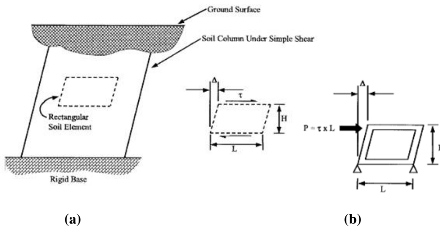
(a) Figure 1. Relative stiffness between soil and a rectangular frame [2]. a) Flexural (shear) distortion of free-field soil medium, b) Flexural (racking) distortion of a rectangular frame
