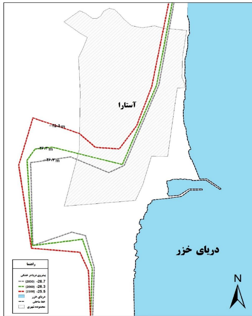
RCP 8.5
