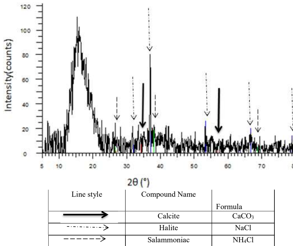
Fig. 4. X-ray diffraction pattern of precipitates collected from isolate 6 cultured on precipitated medium containing 5 % NaCl.
