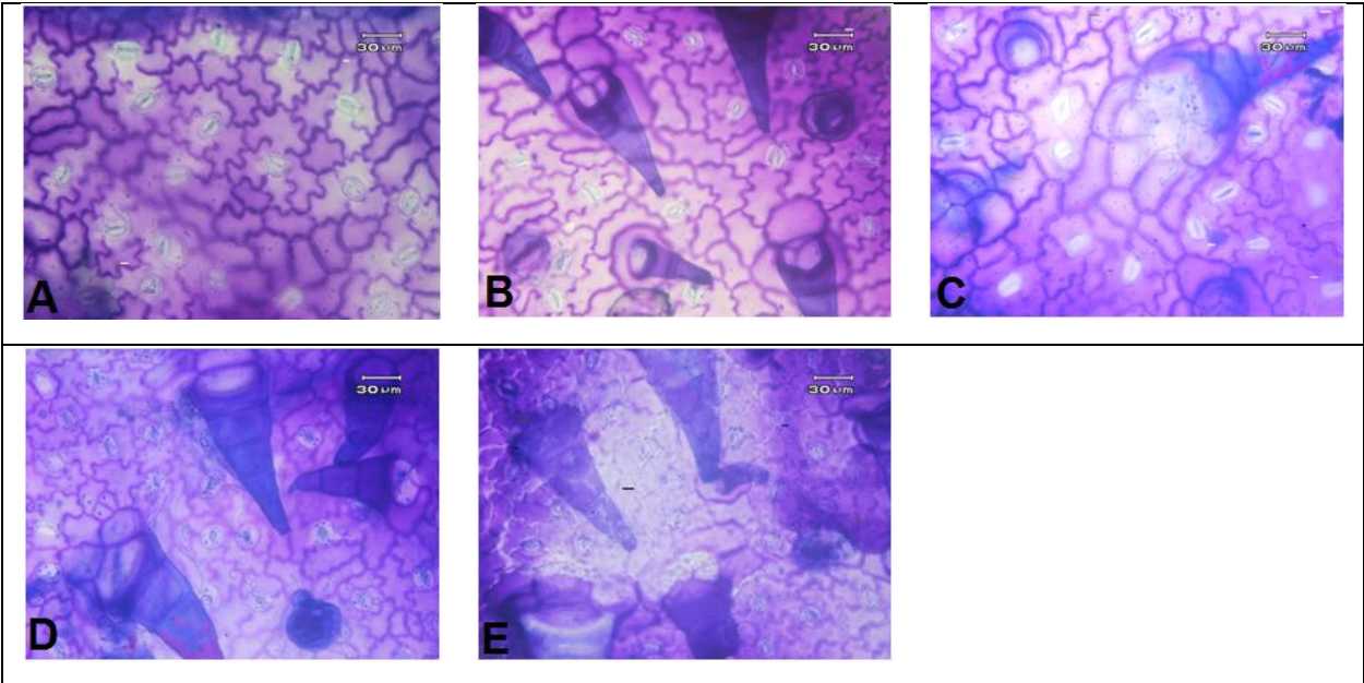
Fig. 5. Upper epidermis of leaf in species studied: A: Zoegeacrinita subsp. baldschuanica ; B: Z. crinita subsp. crinita ; C: Z. crinita subsp. glabricaulis ; D: Z. Lepturea subsp. mianensis ; E: Z. purpurea .
